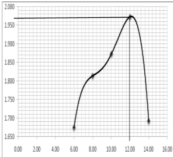
Graph 4.1.3 of Standard Proctor Result From Graph
