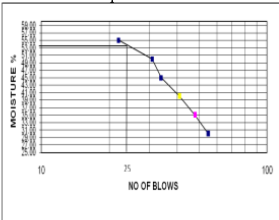
Fig 4.1.2.1: Water content Vs Number of blows.
